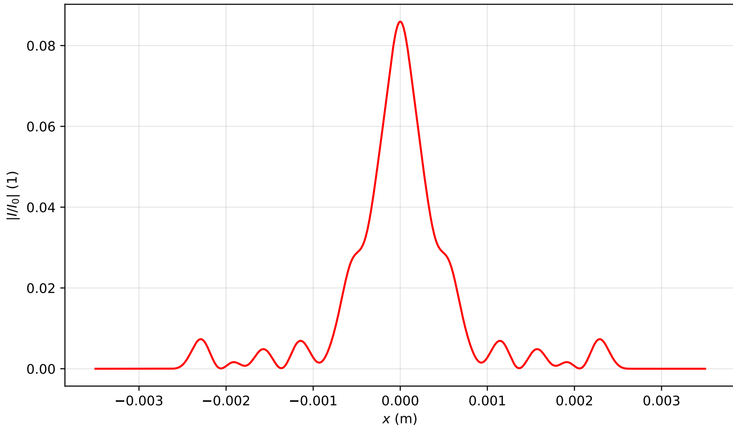
Intensity profile I(x, y = 0, z = 3.981)/I_0 , P_{in}=9.0P_{cr} , artificial time
